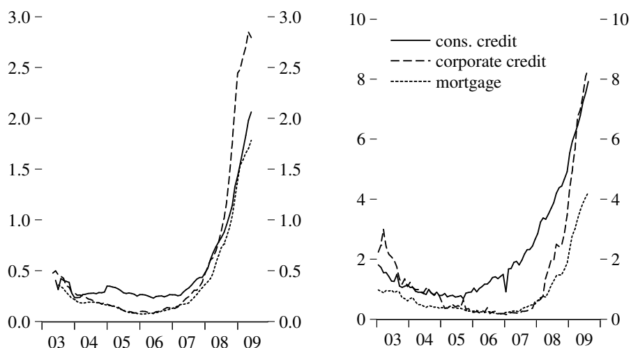
(a) Probability of default rates.
